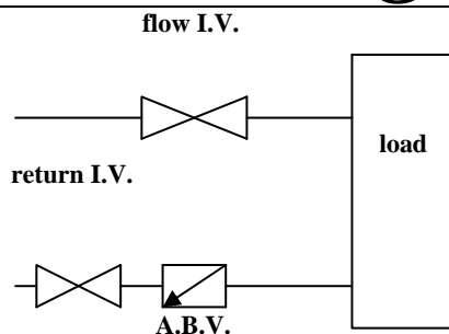
Automatic balancing device in circuit
